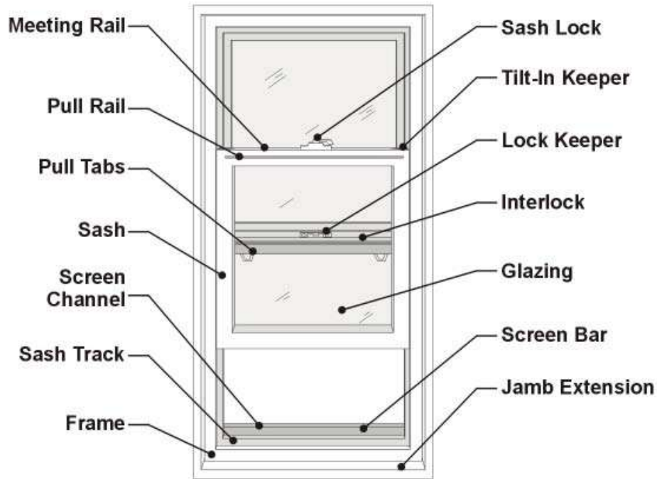
Single Hung (Vertical) (PVC single hung shown)
