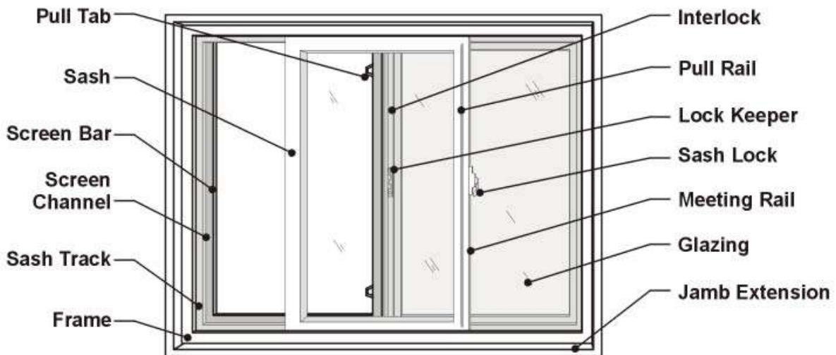
Glider Operator (PVC glider shown)
