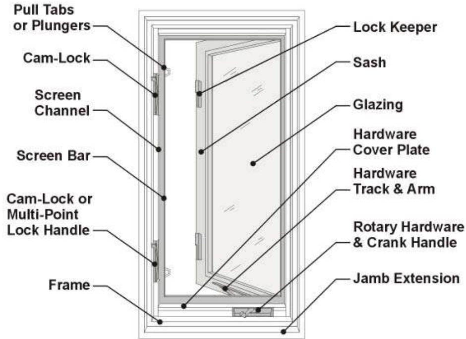
Casement Operator (metal clad wood casement shown)
