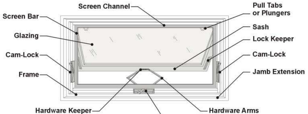
Awning Operator (metal clad wood awning shown)
